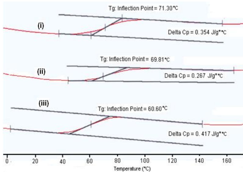
Figure 4. The DSC thermograms for various metal nanoparticles, (i) Cu, (ii) Au and (iii) Ag, in 10% (v/v) epoxy/curing agent (a) first heating and (b) second heating scan.
